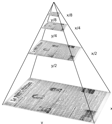
Figure 5: TIFF pyramidal format
